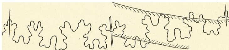
Fig. 5. Suture, Hamites tenawa n. sp., camera lucida drawing.
