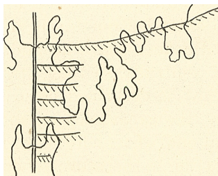
Fig. 3. Suture, Scaphites hilli , n. sp., camera lucida drawing.
