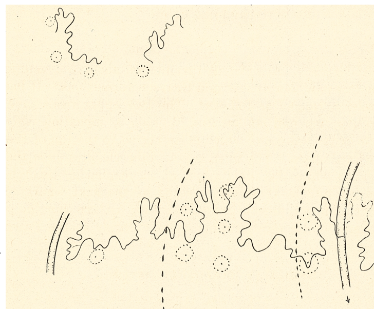
Fig. 6. Suture, Turrilites worthensis n. sp., camera lucida drawing. The upper left hand figure is from the type.
